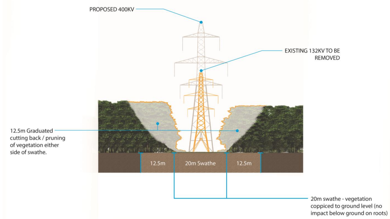
Illustration 7.1 – Sketch of 400kV Overhead Line Construction Within Woodland With an Existing Maintained Swathe
